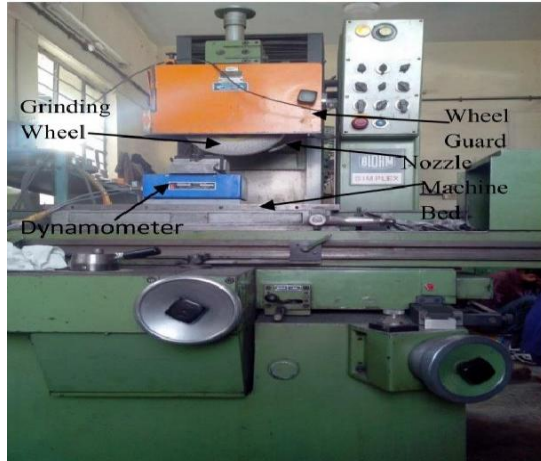
Fig.1 Surface Grinding M/c Setup
