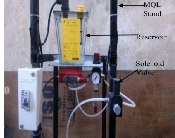
Fig.2 MQL Setup
