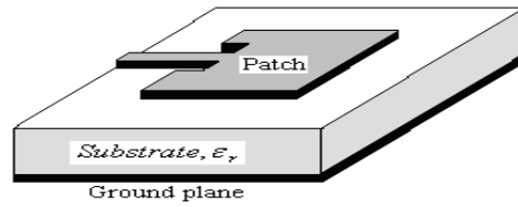
Figure 2.2 Microstrip Line feeding.
