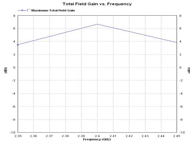
Figure 4.3: Gain of the patch is 6.61 dB at f=2.40002 GHz
