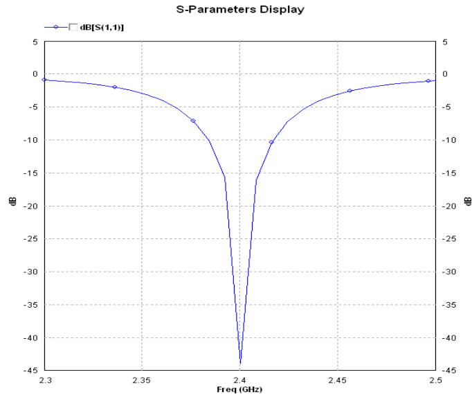
Fig 4.1: Scattering Parameter of a rectangular Patch antenna.
