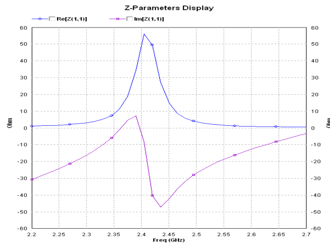
Figure 4.2 Input Impedance of Patch antenna at 2.40582GHz is 50
