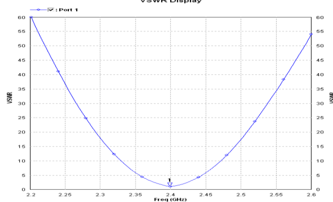
Figure 4.4 VSWR of Microstrip patch antenna is 1.0 at f=2.3995 GHz
