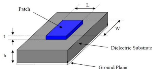
Figure 1.1 Rectangular Microstrip antenna.
