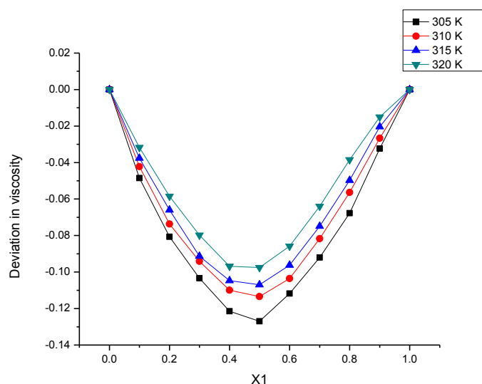
Fig: 4 Plot of Deviation in viscosities v/s X1 for n- butyl acetate and isopropanol
