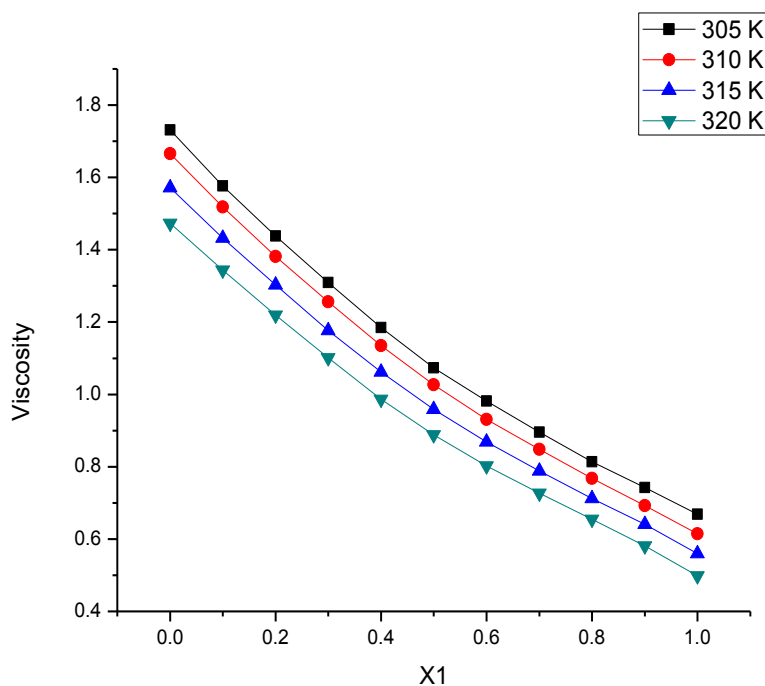
Fig: 3 Plot of Viscosities v/s X1 for n- butyl acetate and isopropanol
