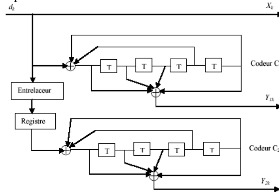
Fig. 1.4 Structural diagram of turbo coder
