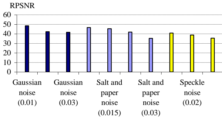
Fig. 1.9 Mean values of RPSNR for 30 test images watermarked and attacked by different Types of Noises
