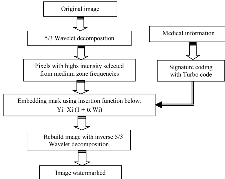
Fig. 1.1 The embedding algorithm
