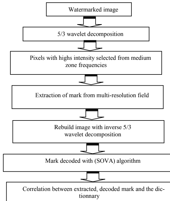
Fig. 1.2 The detection algorithm
