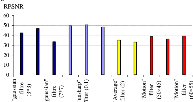
Fig. 1.11. Mean values of RPSNR for 30 tests images Watermarked and attacked by different filters
