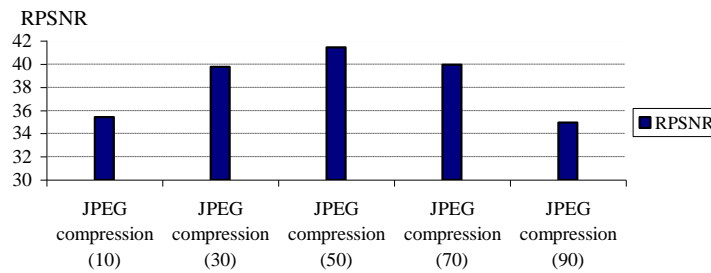
Fig. 1.10. Mean values of RPSNR for 30 test images watermarked and attacked by different ratio of JPEG Compression
