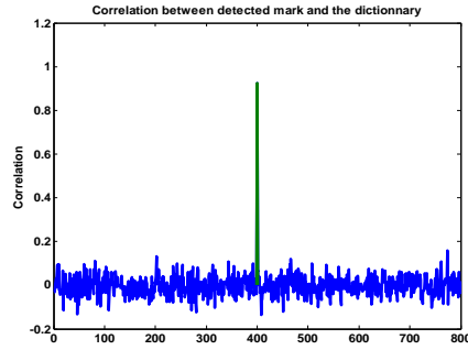
Fig. 1.8. Succeeded detection of a mark after correlation between extracted and decoded mark and the dictionary after Gaussian Filter. Correlation=0. 92
