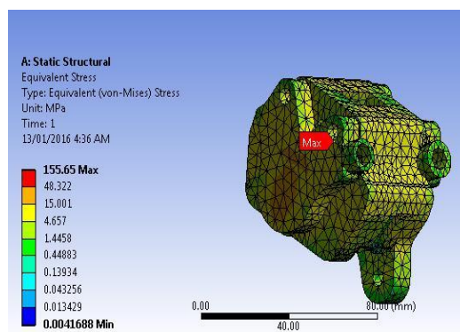
Figure 9 Equivalent stress (von-misses) of a brake caliper
