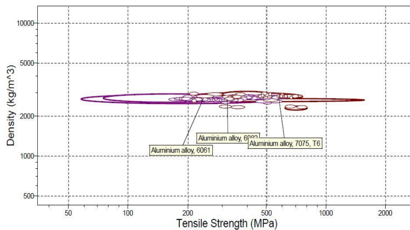
Figure 3 Ashby chart for material selection
