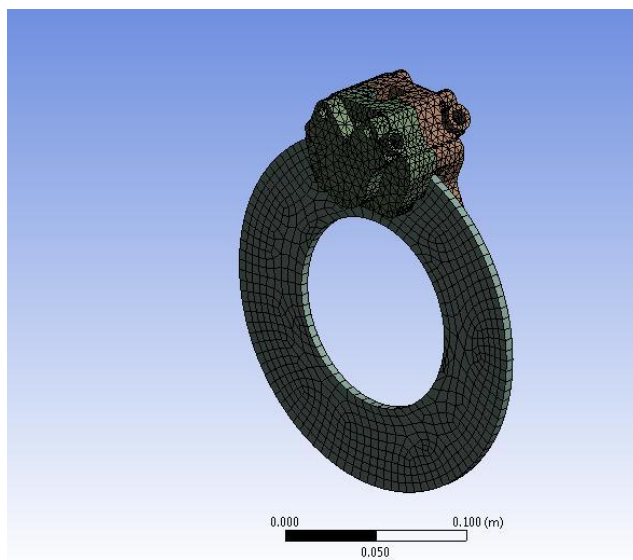
Figure 6 Meshed Model of a Brake Caliper
