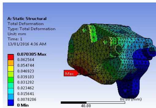
Figure 8 Total deformation of a brake caliper
