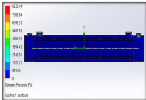
Fig. 4.4: Dynamic Pressure Plot of Finned Tube HX
