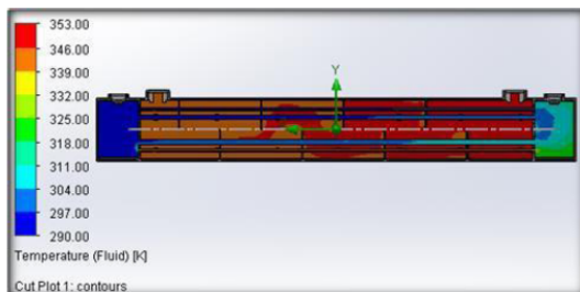
Fig. 4.5: Temperature Plot of Corrugated Tube HX
