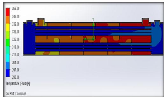
Fig.4.1: Temperature Plot of Smooth Tube HX
