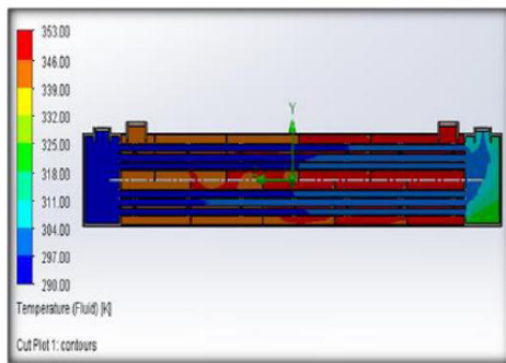
Fig. 4.3: Temperature Plot of Finned Tube HX
