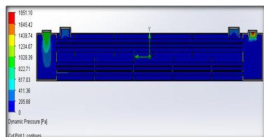
Fig. 4.2: Dynamic Pressure Plot of Smooth Tube HX
